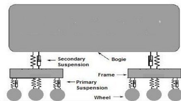
Figure 1: Rail vehicle three wheel engine with primary and secondary suspension system
